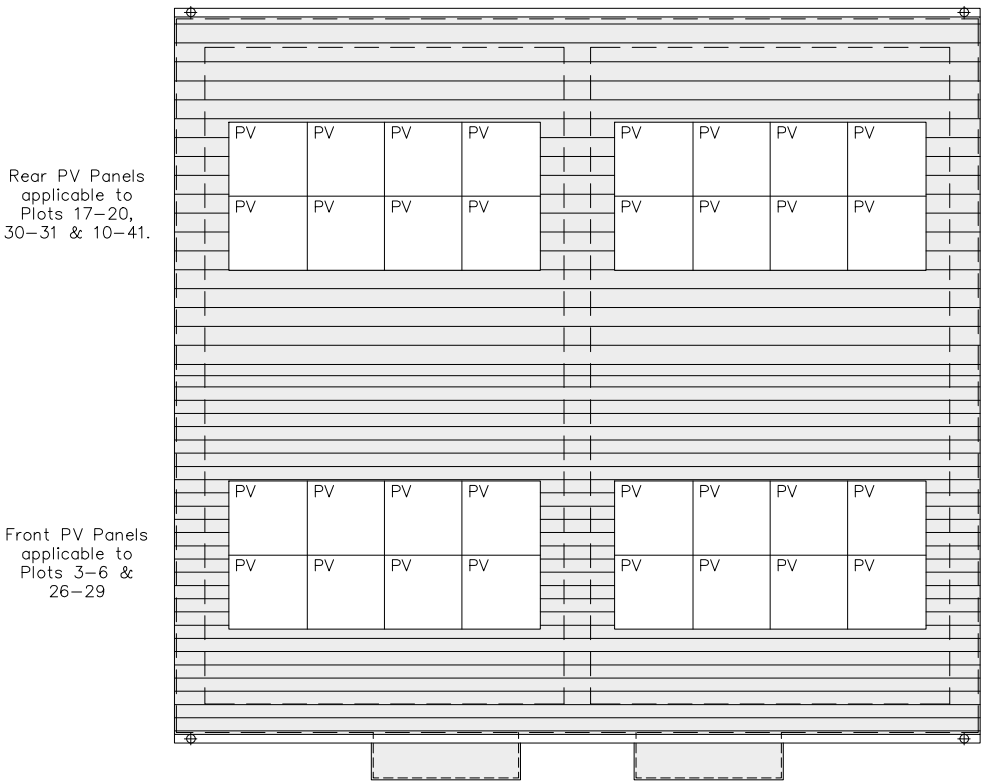
Roof Plan
