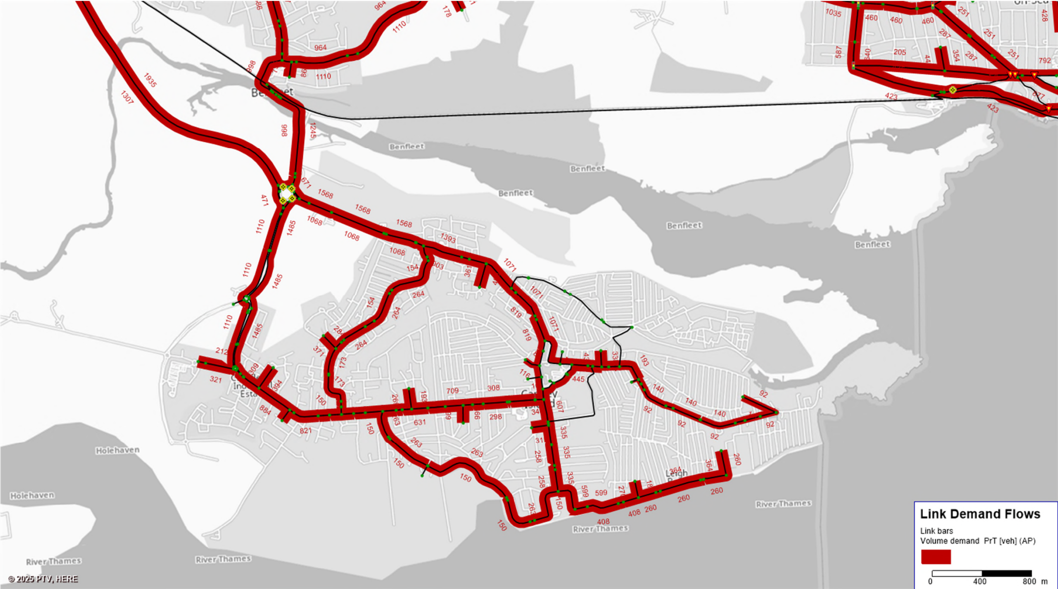
Canvey Island Link Flows PM BAU
